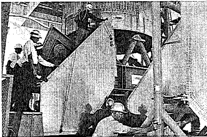
BOLTING FINS TO AFT BODY (NASA Photo S-63-13546)
