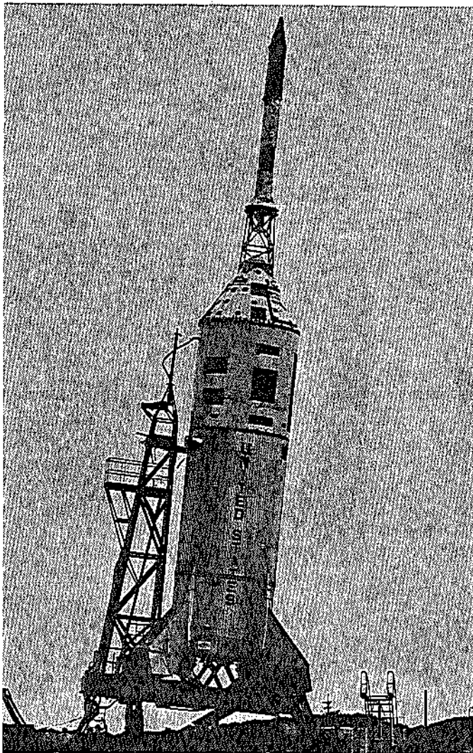
BOILERPLATE-23 ON LAUNCH PAD (NASA Photo S-64-35835)
